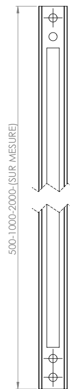
RAIL A1 (RAIL STANDARD)
