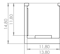
RAIL A1 (RAIL STANDARD)
