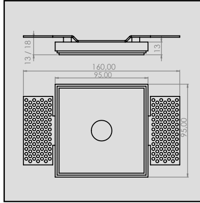
ACSD-RCA-PLA-18 RCA recessed trimless plug Plaster 18mm
