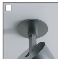
ACS FIPATER 60 XX ENCC Fixing mounting recessed Ø60mm H34mm
