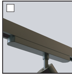
SD015RV 220 0-10V track Width 31mm
